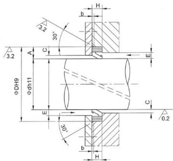
开口式UN旋转油封 Carcoseal/UN/split
