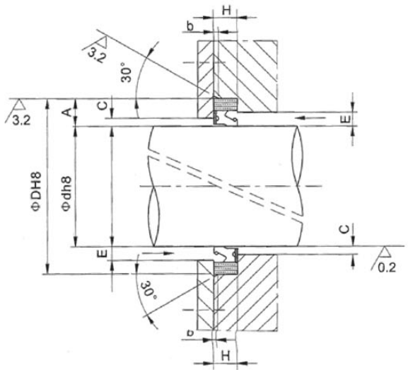
耐压油封Carcoseal/AP
