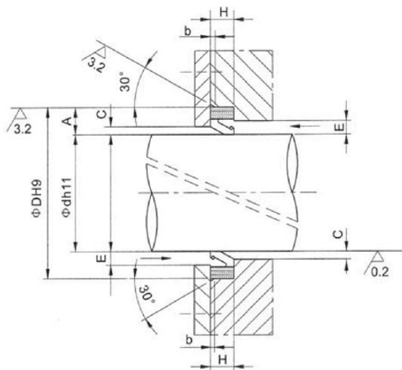
无涵盖安装UN旋转油封 Carcoseal/UN/SF
